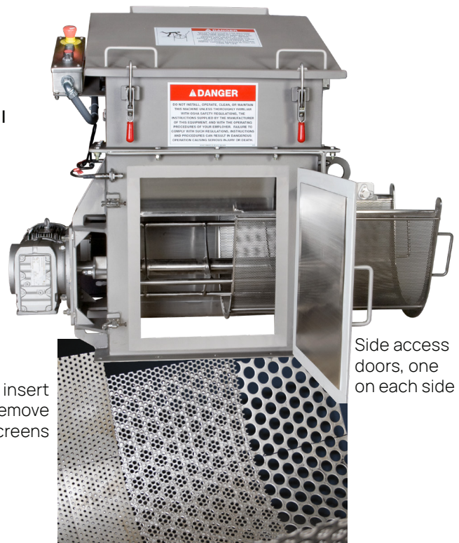
Shown with optional hand-add station with grating, and optional power E-stop & PB station.*
